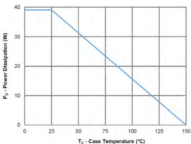
Figure 10: Power Derating
